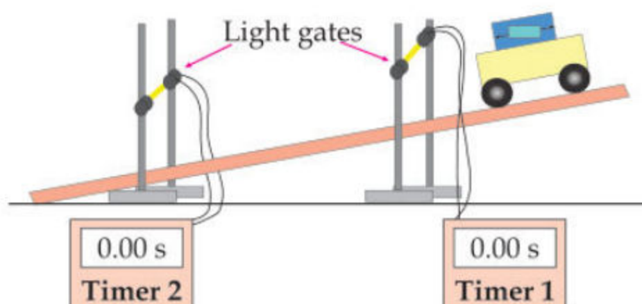
Fig (1.23) Light gates
